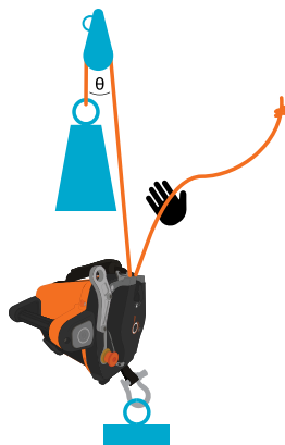
Bottom-rigged Basic setup
